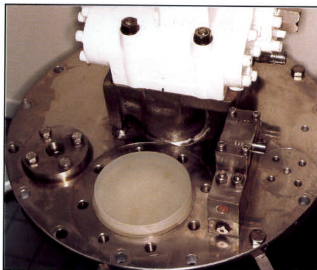
Old design stripping/purging valve fitted on topcover plate.
