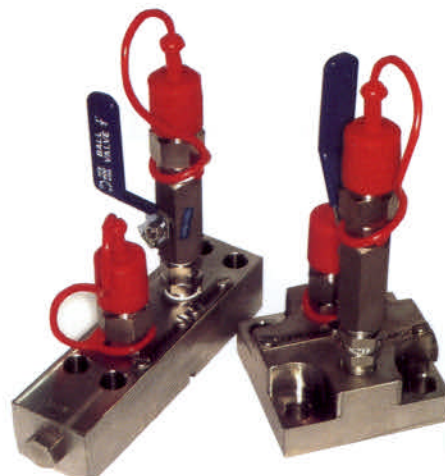
Upgraded stripping/purging valves drg.no.264-363-2 & 293-514-2
