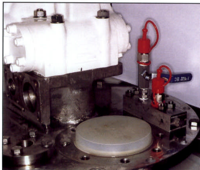
Upgraded stripping/purging valve fitted on topcover plate.
